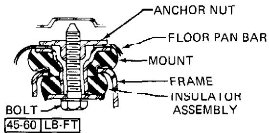
BODY BOLTS 1-2-3-4-6-7
