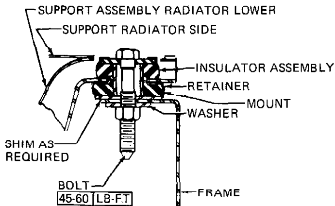
SHEET METAL MOUNT
