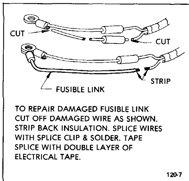
Figure 120-7 Fusible Links
