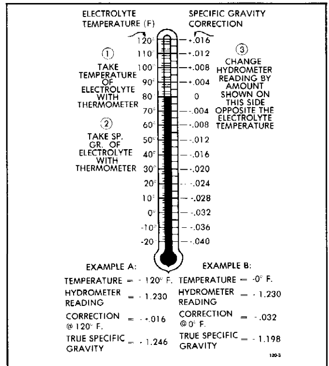
Figure 120-3 Specific Gravity Temperature Correction Scales
