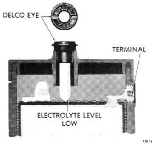
Figure 120-11 Low Electrolyte Level
